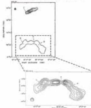
1610-60.5 & 1610-60.8 at 1415 MHz. Galaxies A, B, D & E are identified. (Christiansen, et al. 1977, MNRAS, 181, 183)
