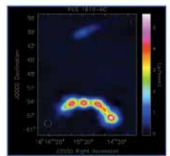
1610-60.5 & 1610-60.8 observed with KAT-7, Aug 2011
